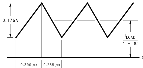
Figure 14. 10 µH Inductor Current, 5 V – 12 V Boost
