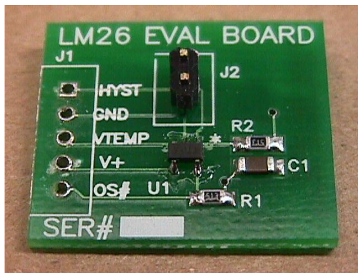
Figure 1. LM26 Evaluation Board
