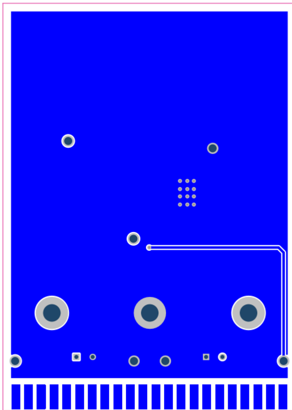
Figure 5. Bottom Layer Routing
