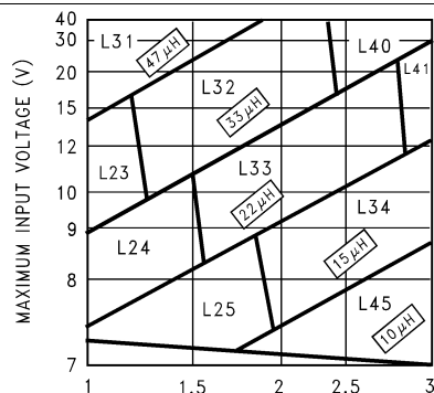
Figure 18. LM2676-5
