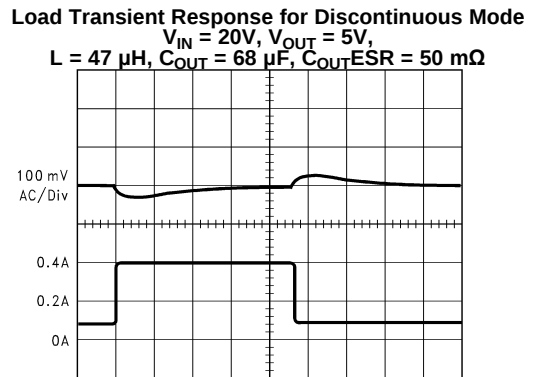
Figure 19. Horizontal Time Base: 1 \mu s /div
