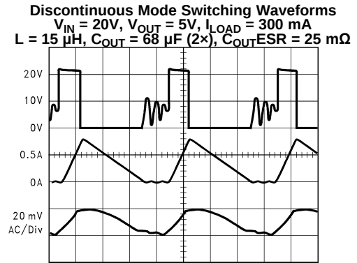
Figure 19. Horizontal Time Base: 1 \mu s /div
