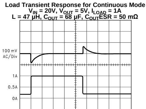
Figure 18. Horizontal Time Base: 1 \mu s /div
