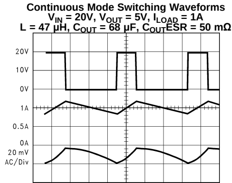
Figure 18. Horizontal Time Base: 1 \mu s /div
