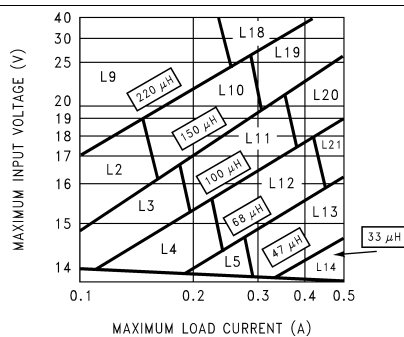
Figure 26. LM2674, 12-V Version
