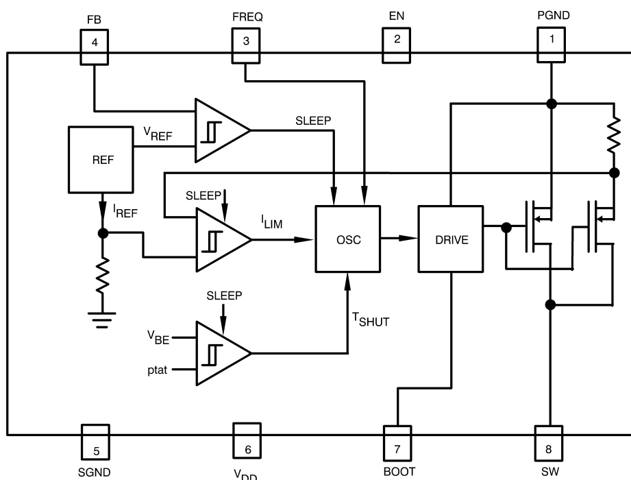
FIGURE 1. Functional Diagram
