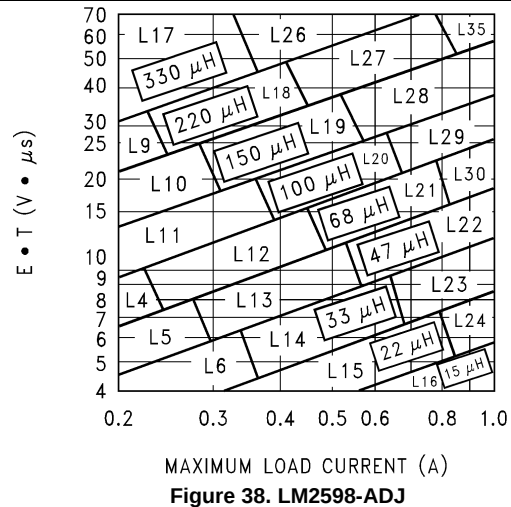
Figure 38. LM2598-ADJ
