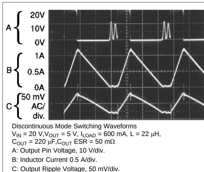
Figure 46. Horizontal Time Base: 2 \mu s/div
