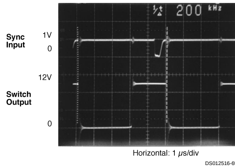
FIGURE 41. Waveforms of a Synchronized 12V Boost Regulator
