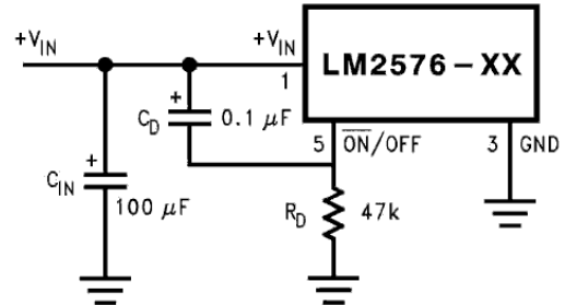
FIGURE 14. Delayed Startup
