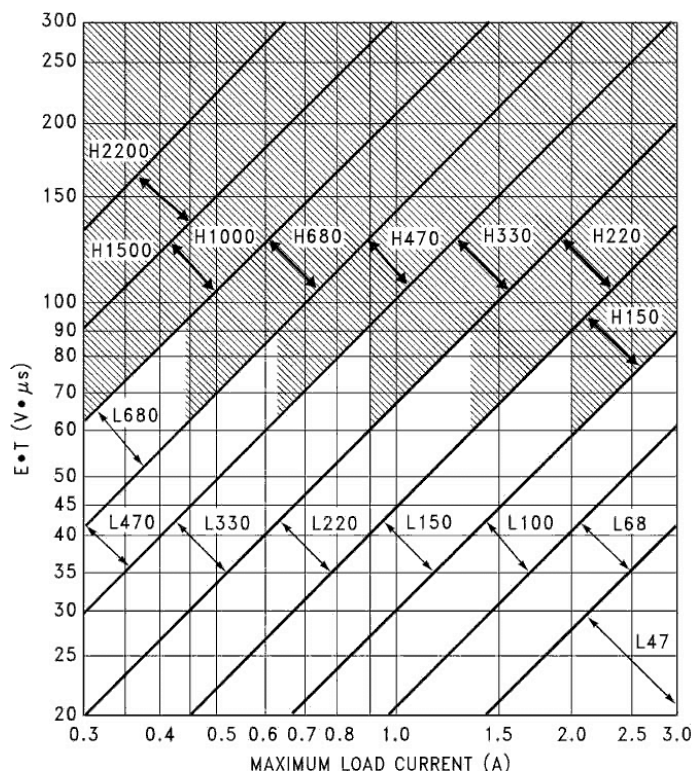
FIGURE 7. LM2576(HV)-ADJ
