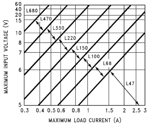
FIGURE 3. LM2576(HV) -3.3
