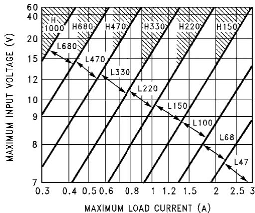
FIGURE 4. LM2576(HV) -5.0
