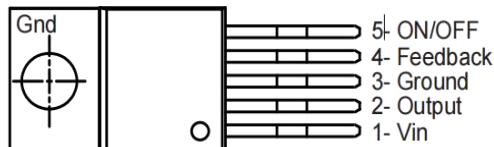
LM2575TB-XX
