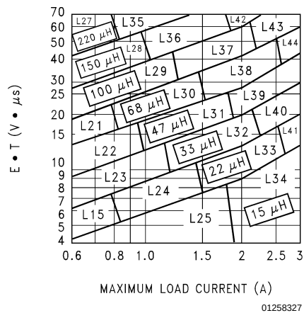
FIGURE 7. LM2575/LM2575HV-ADJ
