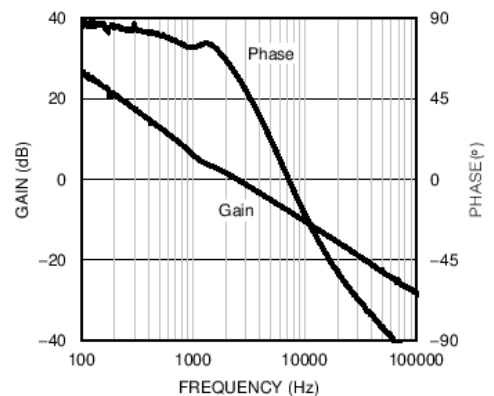
Figure 26. Overall Loop Gain and Phase - Buck-Boost Mode
