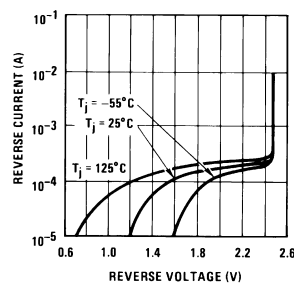
Reverse Characteristics
