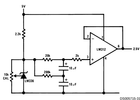
Low Noise Buffered Reference
