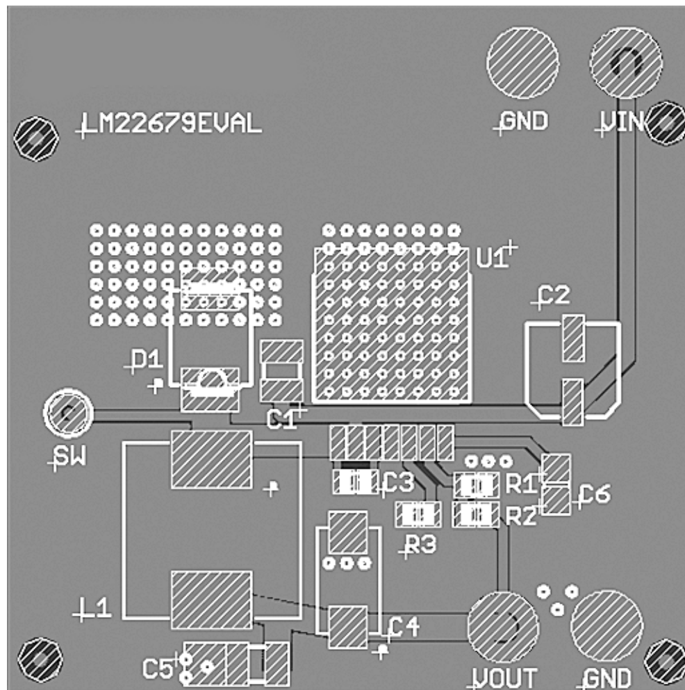
Figure 17. LM22679 Layout Example
