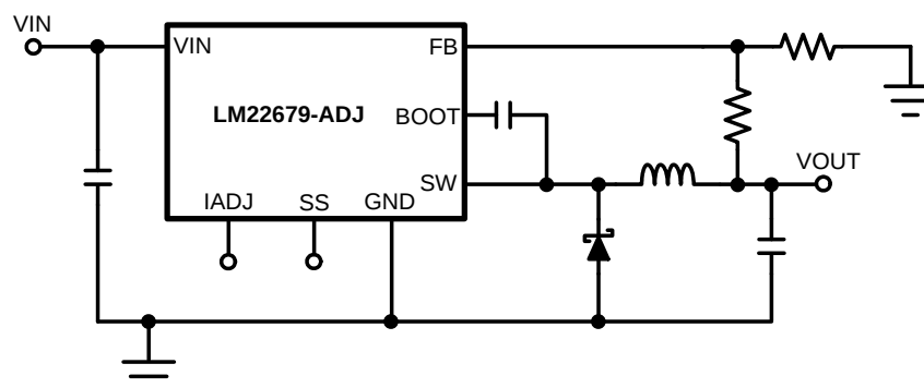
Simplified Application Schematic
