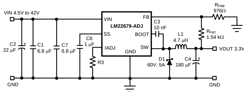
Figure 14. Typical Buck Regulator Application
