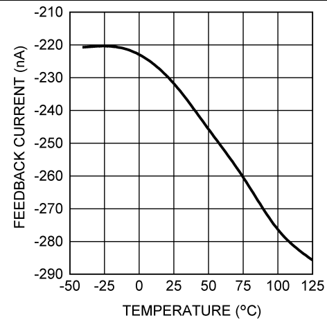
Figure 4. Feedback Bias Current vs Temperature
