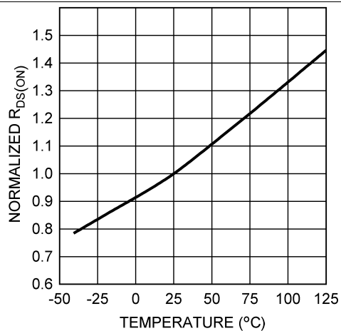
Figure 6. Normalized R_{DS(on)} vs Temperature
