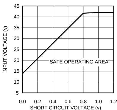
Figure 17. SOA at 800 kHz
