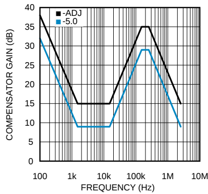
Figure 14. Compensator Gain
