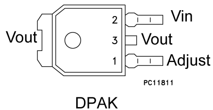
Figure 2. Pin connections (top view)
