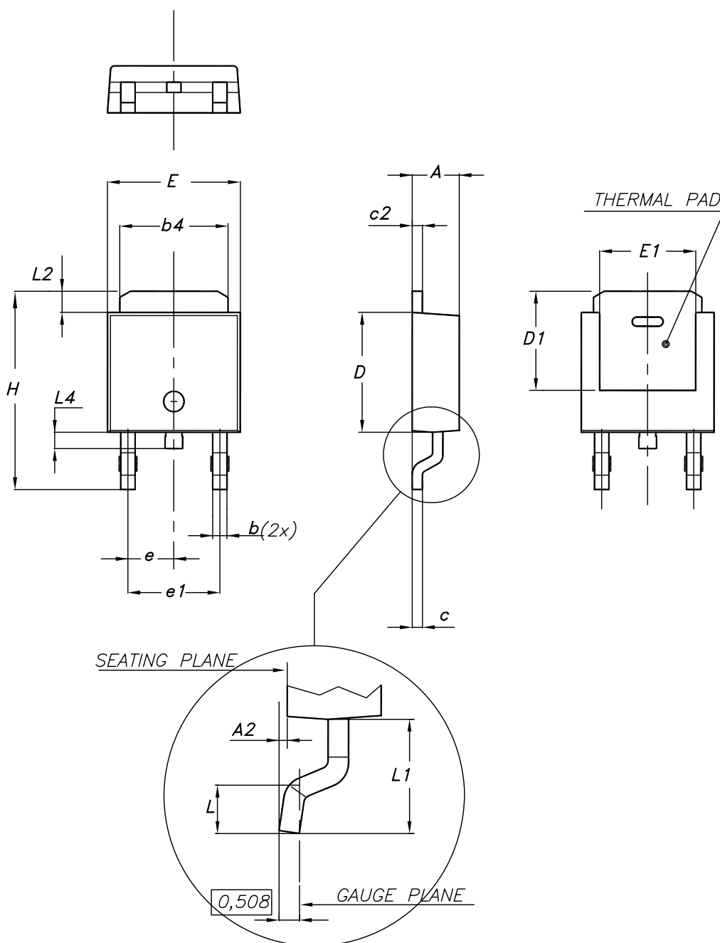
Figure 14. DPAK (TO-252) package outline E
