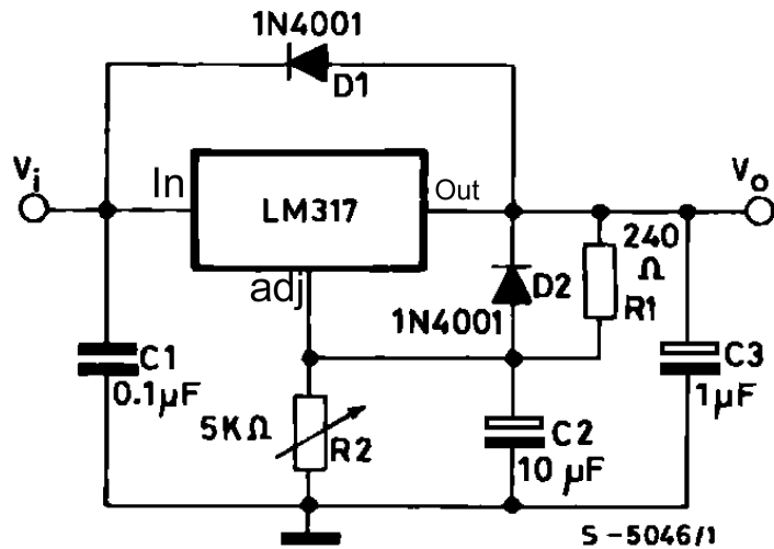
Figure 8. Voltage regulator with protection diodes
