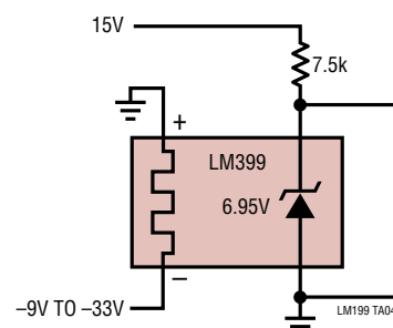
Negative Heater Supply with Positive Reference
