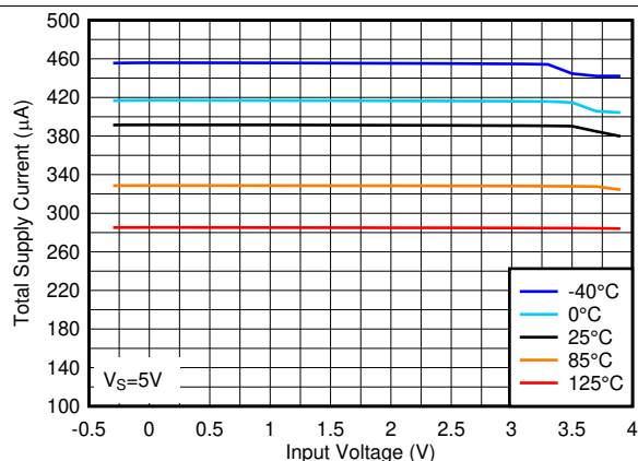
Figure 9. Total Supply Current vs. Input Voltage at 5V
