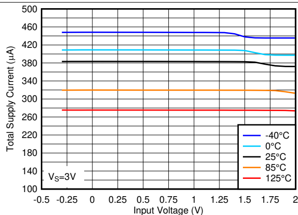
Figure 7. Total Supply Current vs. Input Voltage at 3V
