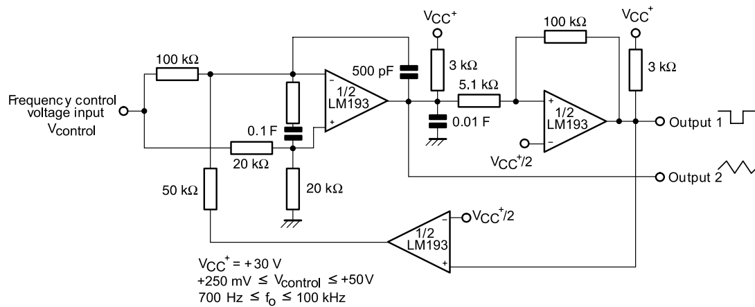
Figure 20: Two-decade, high-frequency VCO
