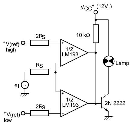
Figure 16: Limit comparator
