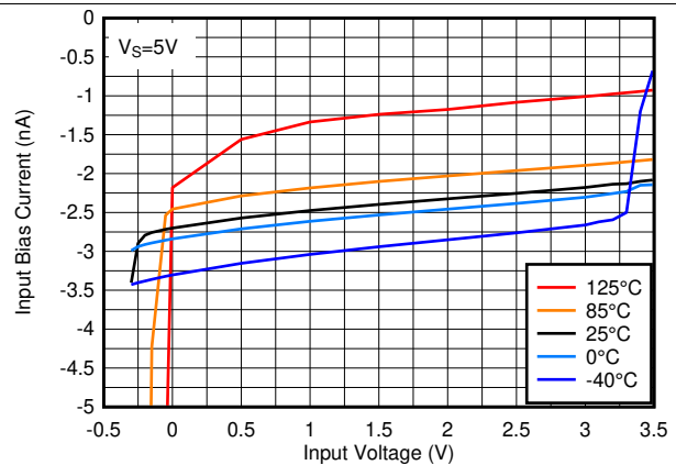
Figure 21. Input Bias Current vs. Input Voltage at 5V
