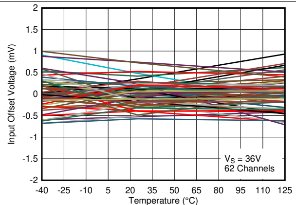
Figure 15. Input Offset Voltage vs. Temperature at 36
