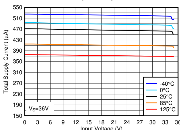
Figure 11. Total Supply Current vs. Input Voltage at 36V
