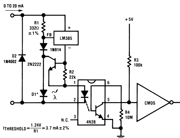
Figure 31. Precision Floating Current Detector
