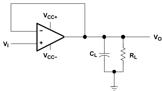
Figure 49. Unity-Gain Amplifier
