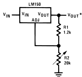
Figure 33. 1.2V–20V Regulator with Minimum Program Current
