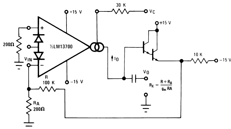
Figure 29. Voltage Controlled Resistor, Single-Ended
