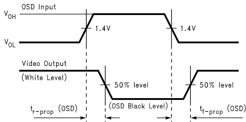
Figure 3. OSD Propagation Delays
