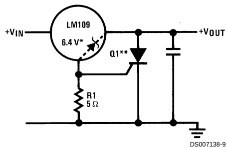
Output Crowbar
