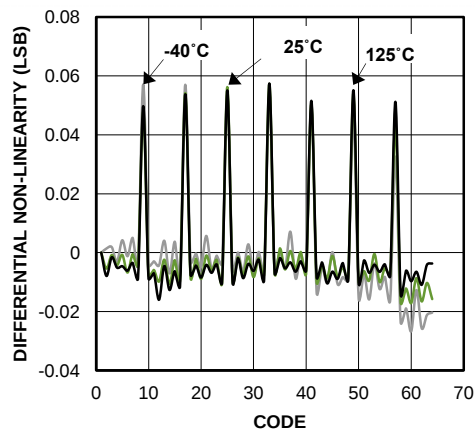
Figure 10. Differential Non-Linearity
