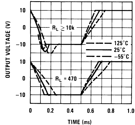
Figure 18. Follower Pulse Response
