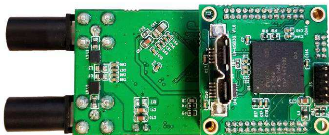
Back View
