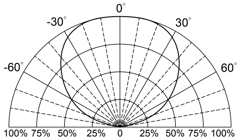
Fig.3 Directivity Radiation
