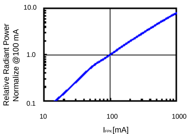
Fig.4 Relative Radiant Power vs. Forward Peak Current
