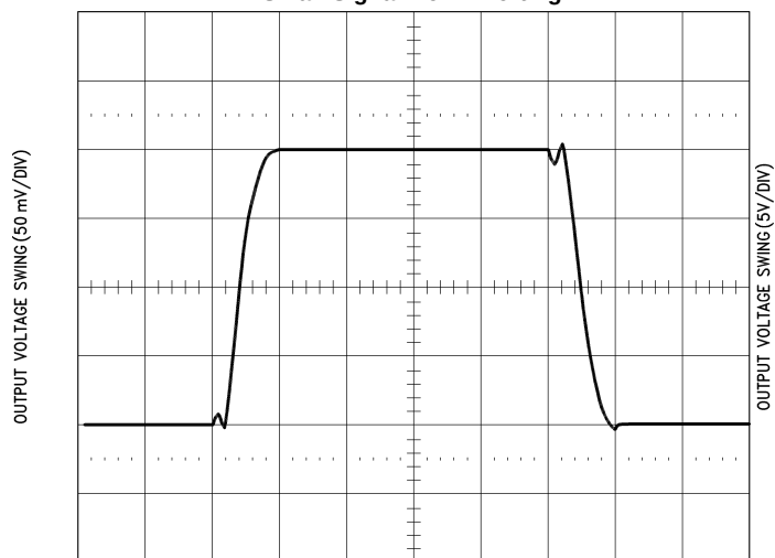
TIME (0.5 μs/DIV) Figure 26.
