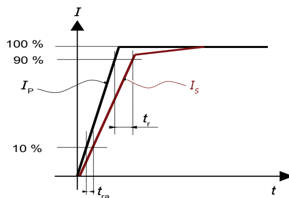
Figure 6: Response time t_r and reaction time t_{ra}
