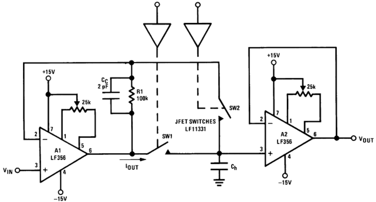
Figure 51. Fast Sample and Hold
