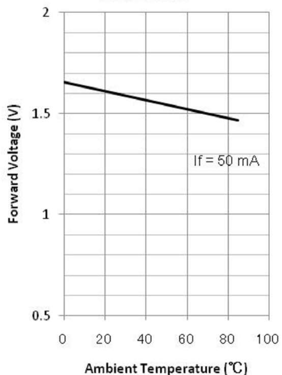
Forward Voltage - Ambient Temperature
