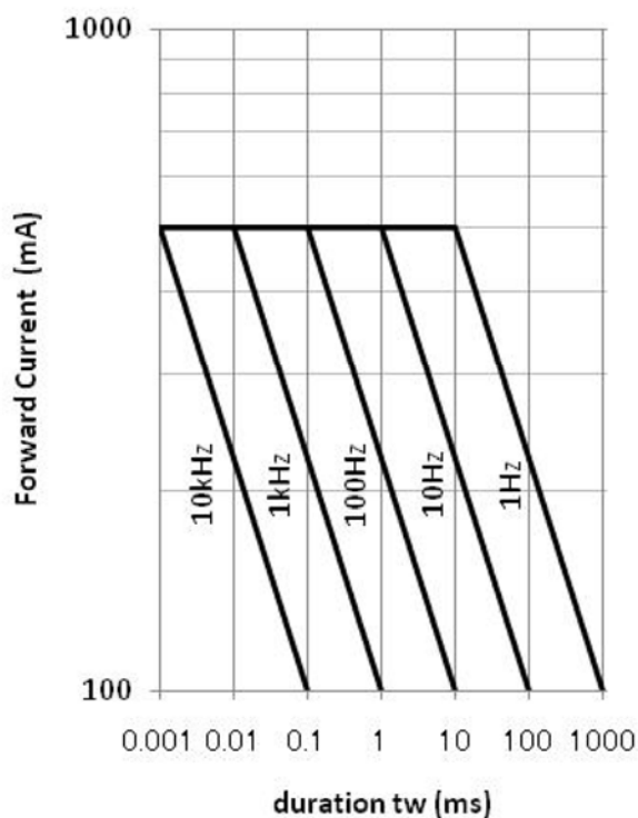
Forward Current - Pulse Duration
