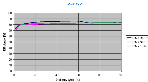
Figure 24. Efficiency versus DIM duty cycle, V_{IN} = 12\text{ V} , 6 rows, 10 white LEDs (60 mA) in series, F_{SW} = 660\text{ kHz}
