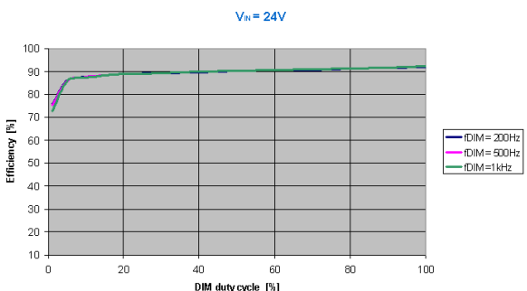
Figure 27. Efficiency versus DIM duty cycle, V_{IN} = 24\text{ V} , 6 rows, 10 white LEDs (60 mA) in series, F_{SW} = 825\text{ kHz}
