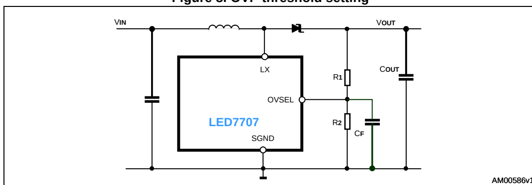
Figure 8. OVP threshold setting
