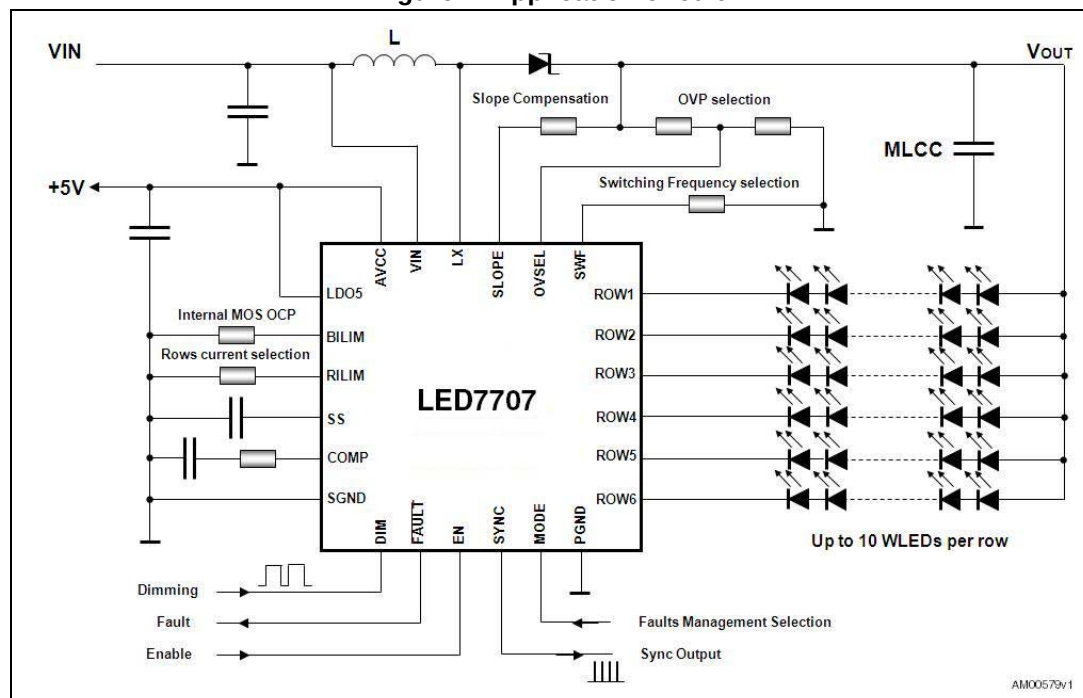
Figure 1. Application circuit
