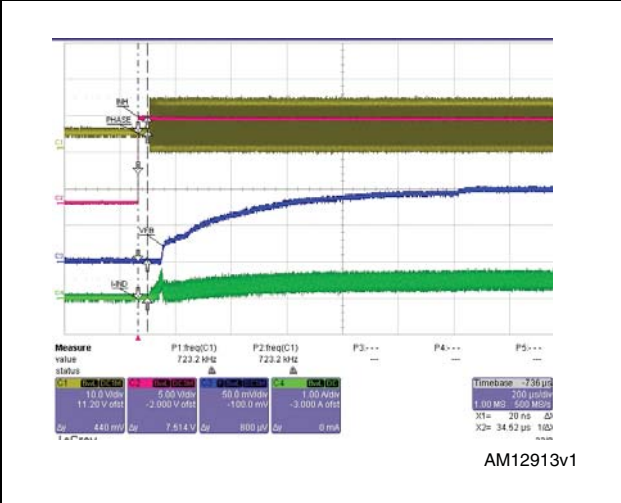
Figure 26. Dimming operation
