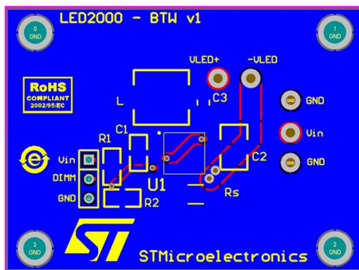
Figure 23. PCB layout (bottom side) SO8 package
