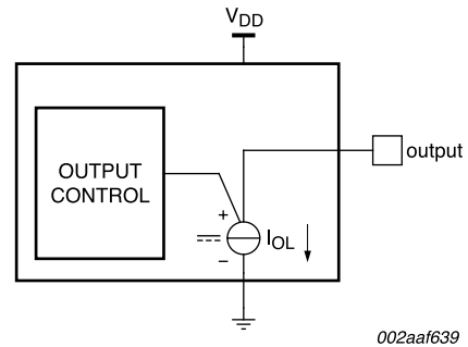
(b) Example Constant-Current Output Structure
