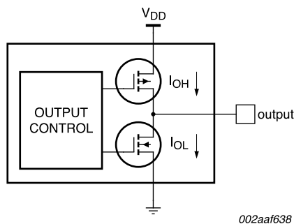
(a) Example Voltage-Switch Output Structure
