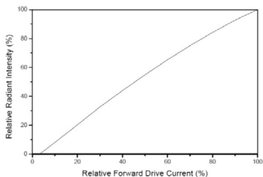
Output Power vs. Forward Current
