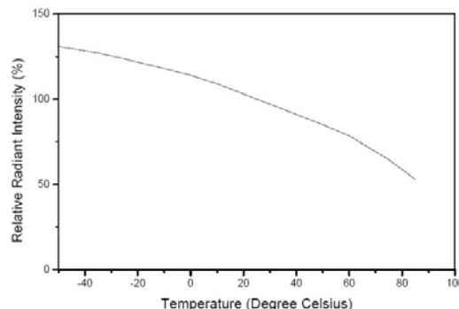
Output Power vs. Temperature
