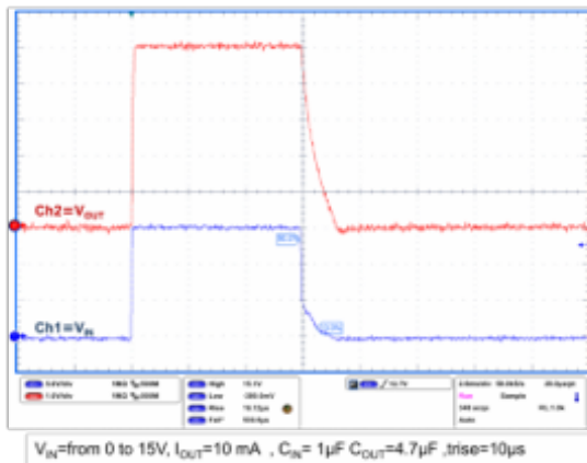
Figure 22. Turn-on time ( V_{OUT} = 5\text{ V} )
