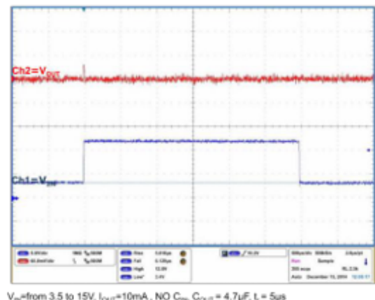
Figure 25. Line transient ( V_{OUT} = 1.2\text{ V} )
