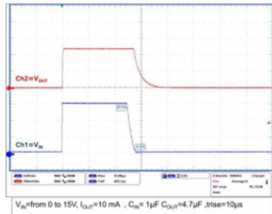
Figure 23. Turn-on time ( V_{OUT} = 1.2\text{ V} )
