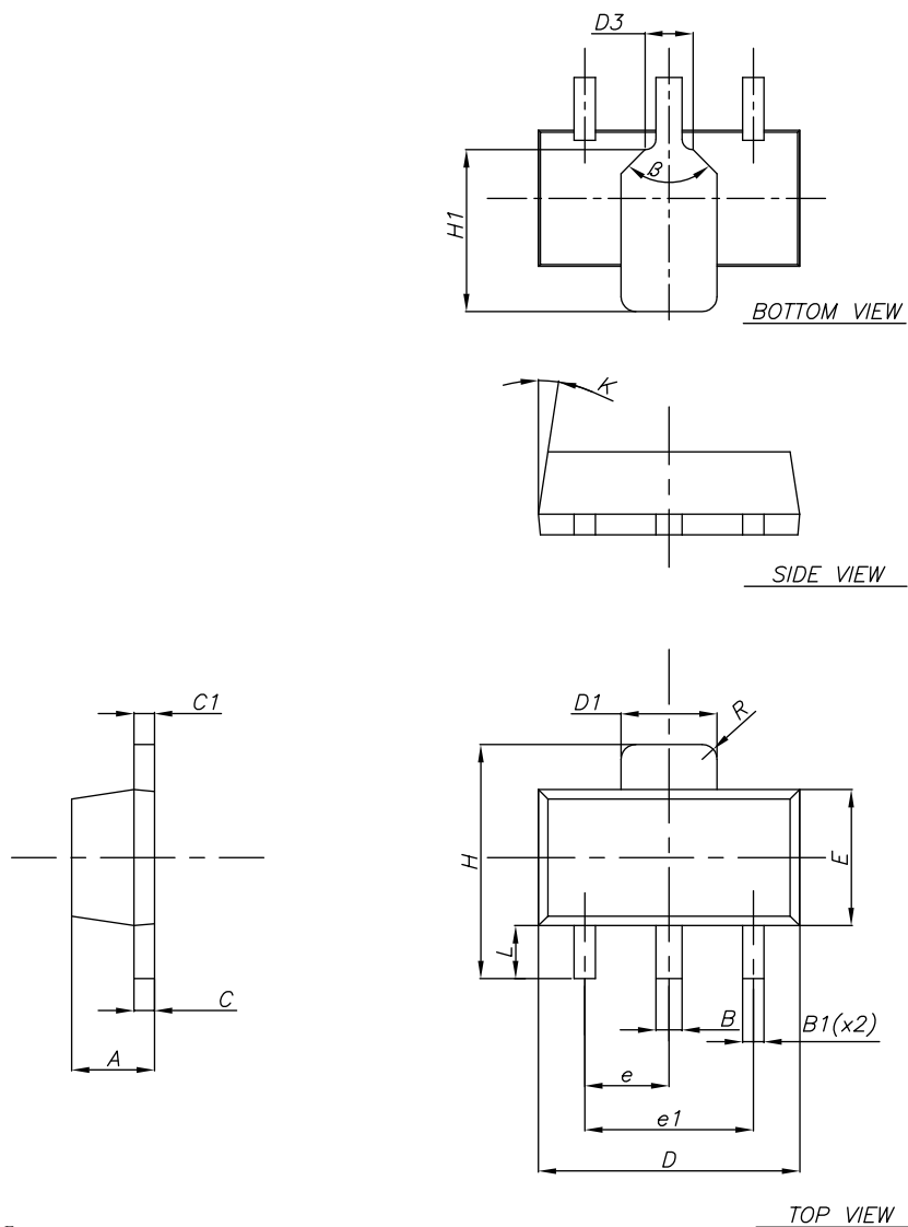
Figure 38. SOT-89 package outline
