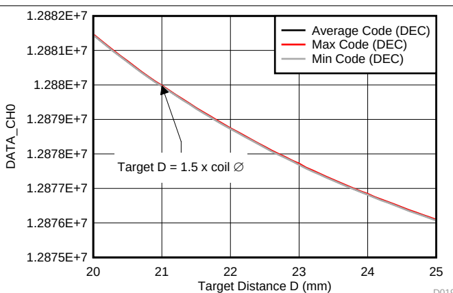
Figure 63. Output Code vs. Target Distance (20 to 25mm)
