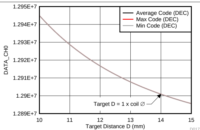
Figure 61. Output Code vs. Target Distance (10 to 15mm)
