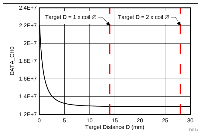
Figure 58. Output Code vs. Target Distance (0 to 30mm)
