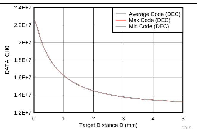
Figure 59. Output Code vs. Target Distance (0 to 5mm)
