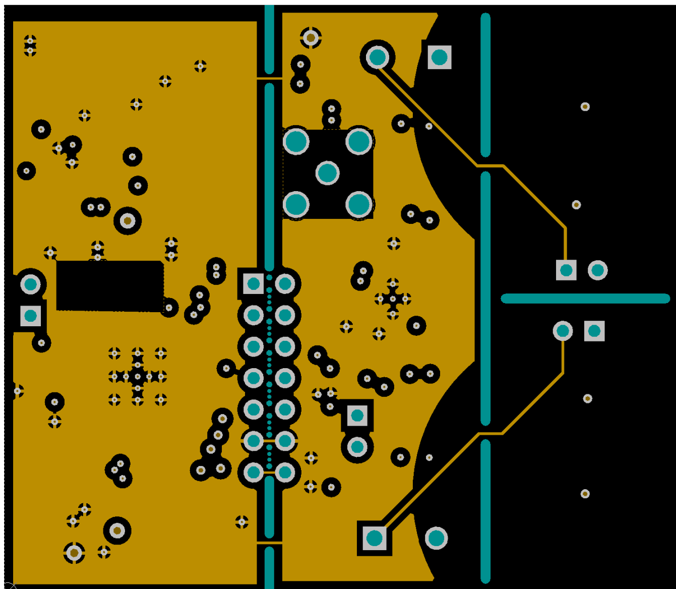
Figure 47. LDC1312/1612 Layout MidLayer 1 – Ground Plane
