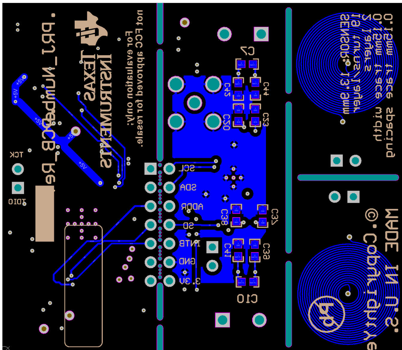
Figure 49. LDC1312/1612 Layout Bottom Layer – Signals Plane
