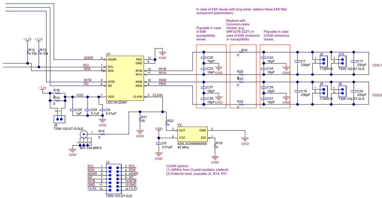
Figure 44. LDC1312/1612
