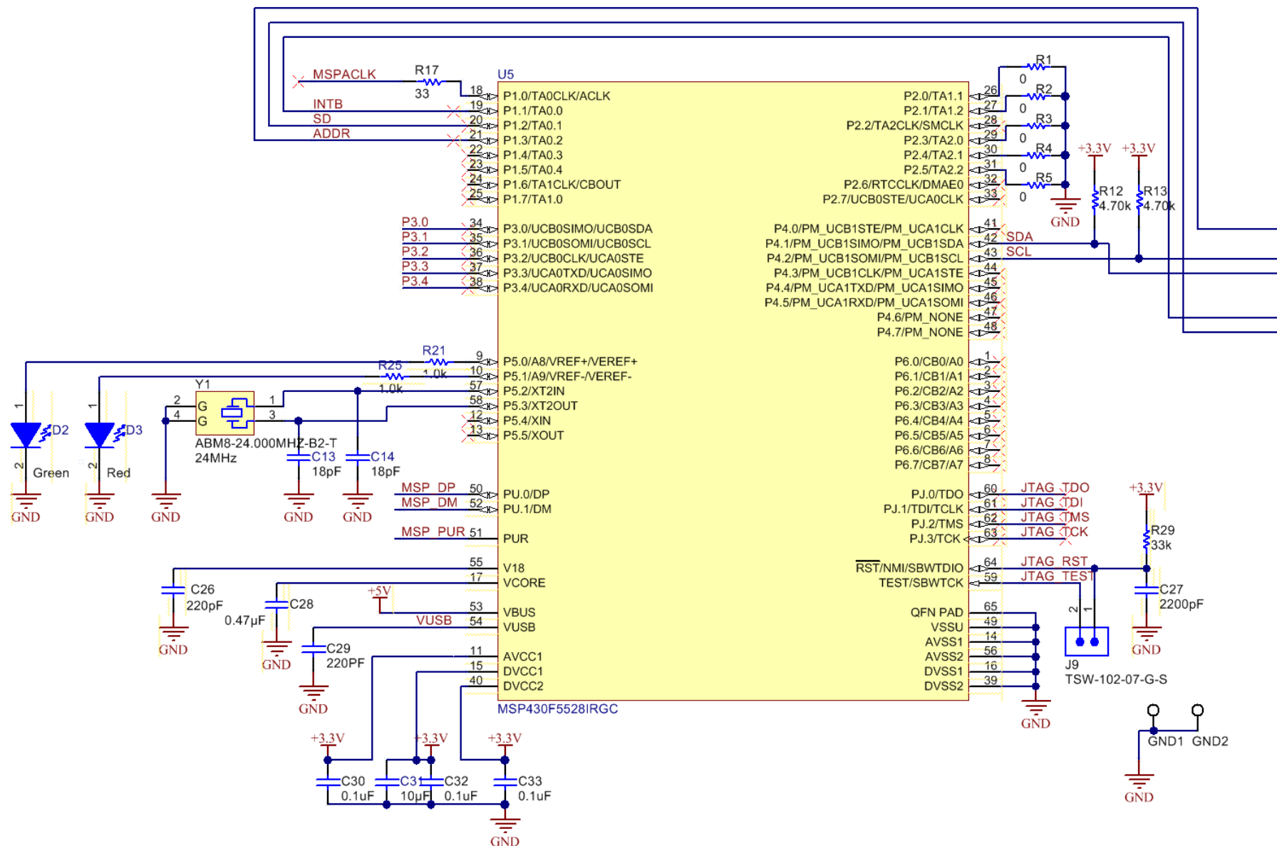
Figure 45. LDC1312/1612 MSP430 Connections
