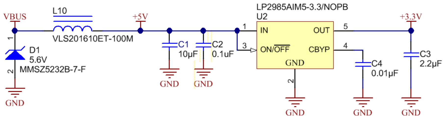
Figure 43. LDC1312/1612 Power Circuit
