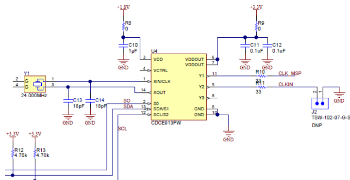
Figure 60. LDC1312/1612 REV A Clocking
