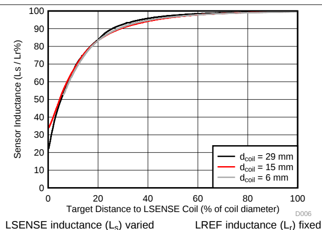
Figure 8. Inductance vs. Distance
