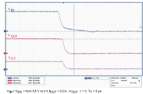
Figure 21: Turn-off time ( V_{OUT} = 1 V )
