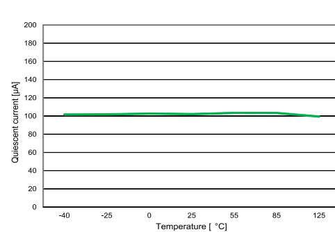
Figure 9: Quiescent current vs temperature ( I_{OUT} = 200 \text{ mA} )
