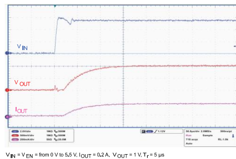
Figure 20: Turn-on time ( V_{OUT} = 1 V )
