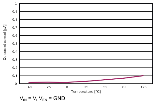
Figure 10: Shutdown current vs temperature
