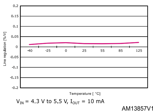
Figure 6: Line regulation vs temperature
