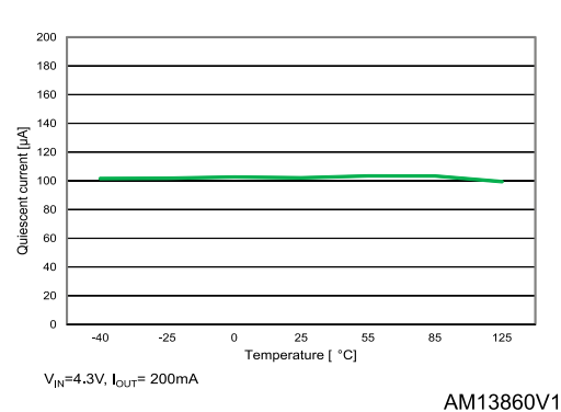
Figure 9: Quiescent current vs temperature ( I_{OUT} = 200 \text{ mA} )
