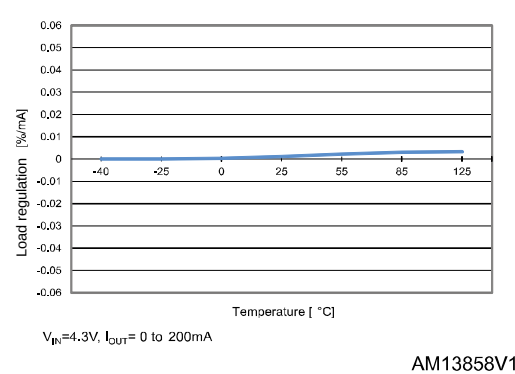
Figure 7: Load regulation vs temperature
