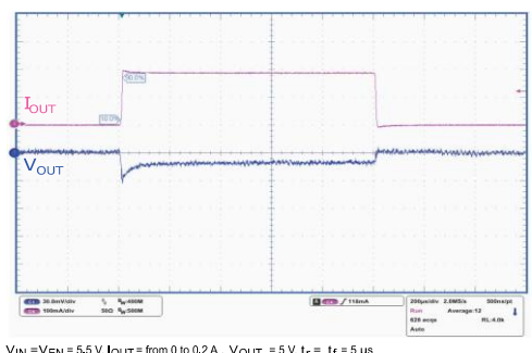
Figure 27: Load transient ( V_{OUT} = 5\text{ V} )
