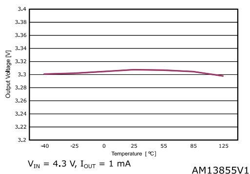
Figure 4: Output voltage vs temperature ( I_{OUT} = 1 \text{ mA} )
