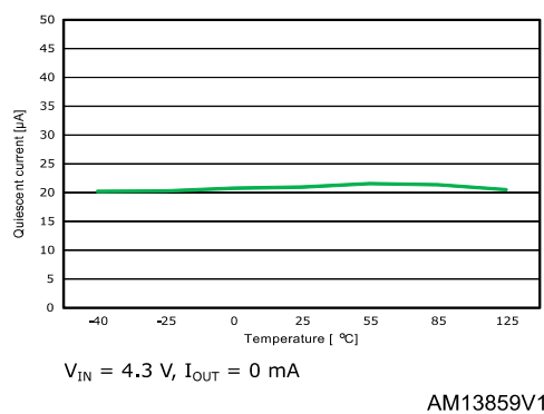
Figure 8: Quiescent current vs temperature ( I_{OUT} = 0 \text{ mA} )
