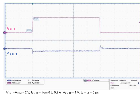
Figure 26: Load transient ( V_{OUT} = 1\text{ V} )
