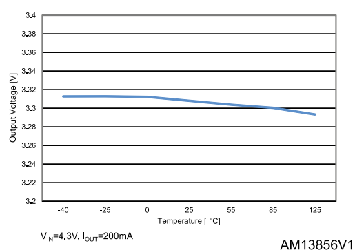
Figure 5: Output voltage vs temperature ( I_{OUT} = 200 \text{ mA} )
