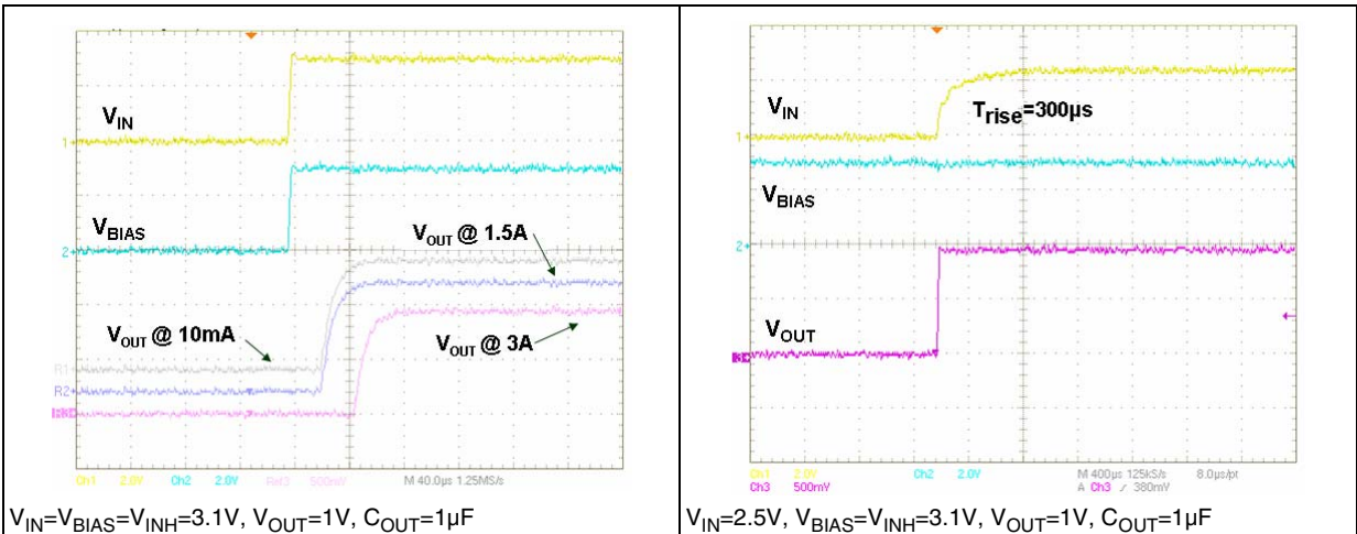
Figure 21. V_{BIAS} & V_{IN} Start Up transient response ( V_{IN} and V_{BIAS} Start Up at the same time) Figure 22. V_{IN} Start Up transient response ( V_{BIAS} Start Up before V_{IN} )
