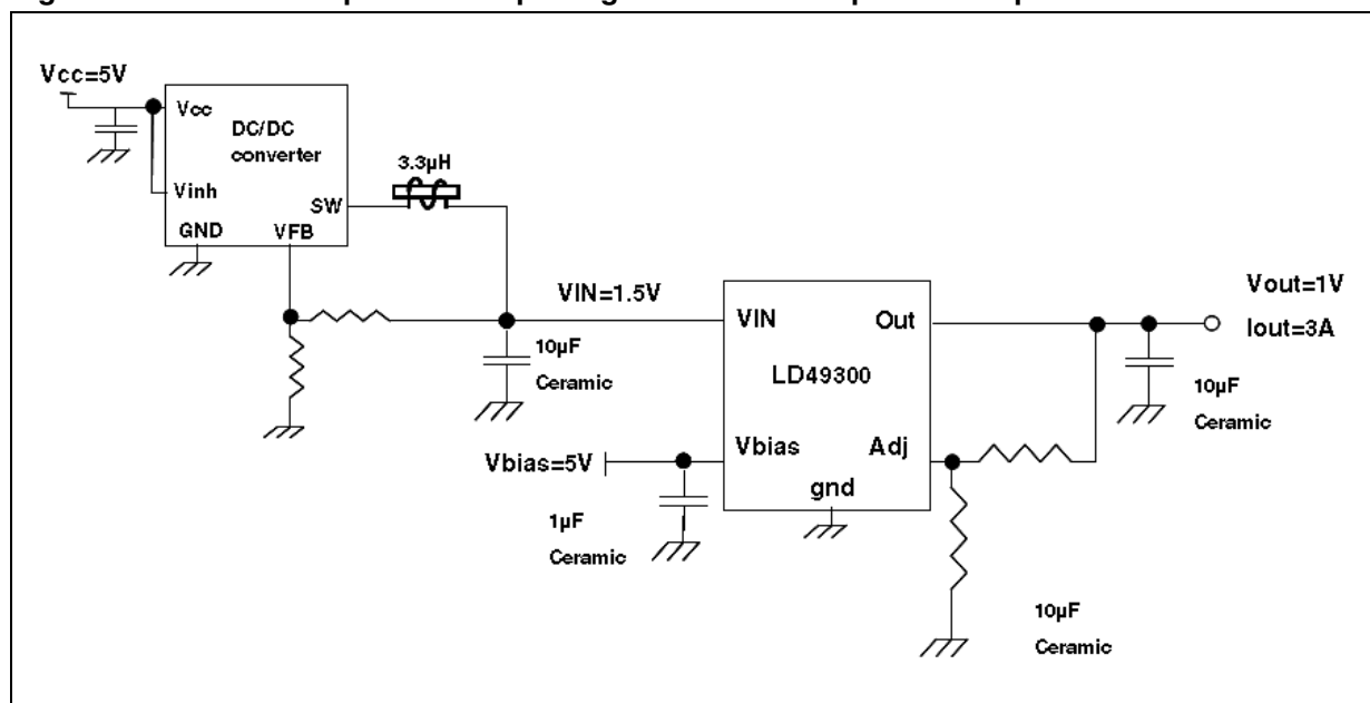
Figure 4. LD49300xx plus DC-DC pre-regulator to reduce power dissipation
