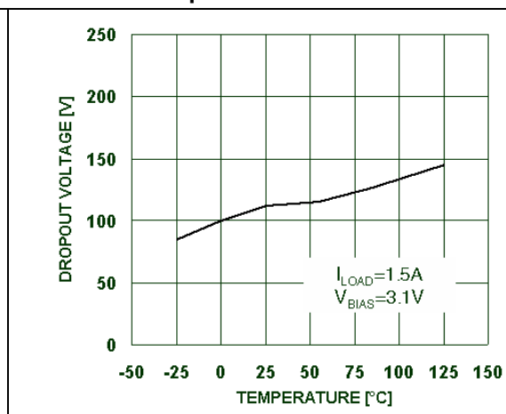
Figure 12. Dropout voltage ( V_{IN}-V_{OUT} ) vs. temperature
