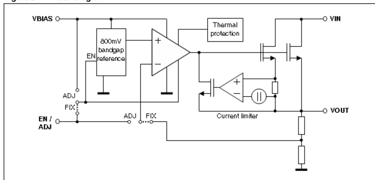
Figure 6. Block diagram
