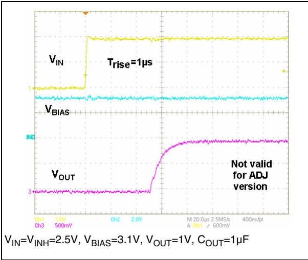
Figure 23. V_{IN} start up transient response ( V_{BIAS} start up before V_{IN} and V_{INH} = V_{IN} )
