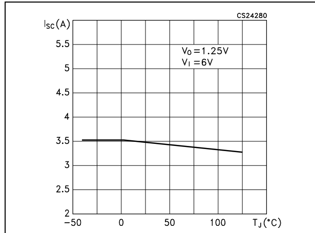
Figure 13. Short circuit current vs temperature
