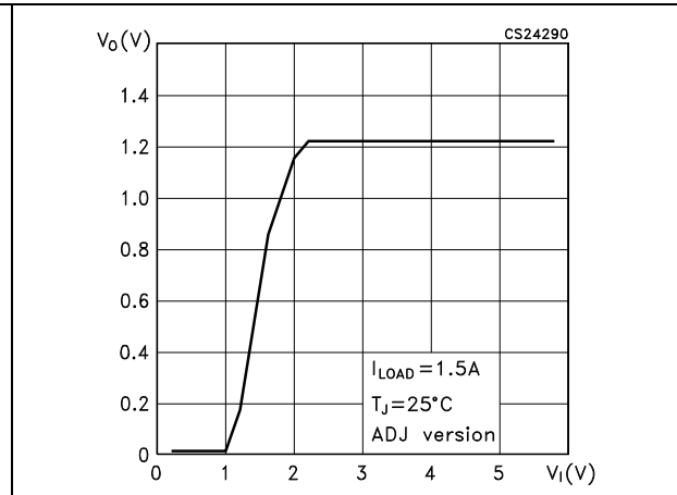
Figure 14. Output voltage vs input voltage
